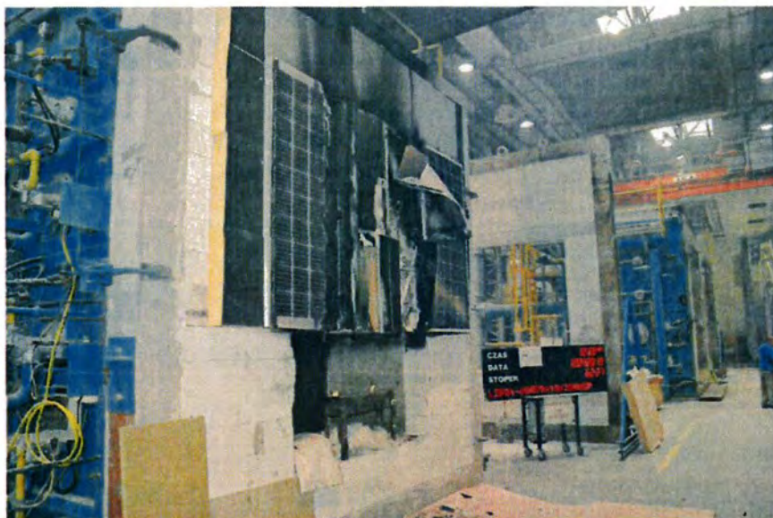
Fig. 41. View of the test element right after the test
