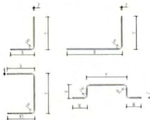
Fig. 2 Stainless AGS brackets, type 28
