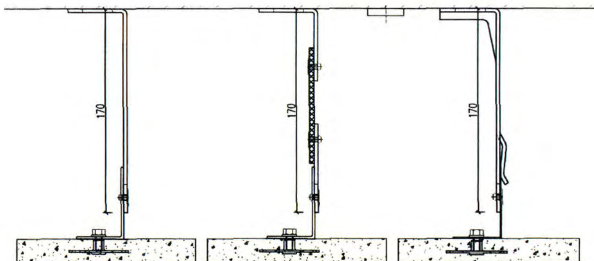
Fig. 12. Details of test elements – details: mounting of GRC panels to substructures in comparative tests
